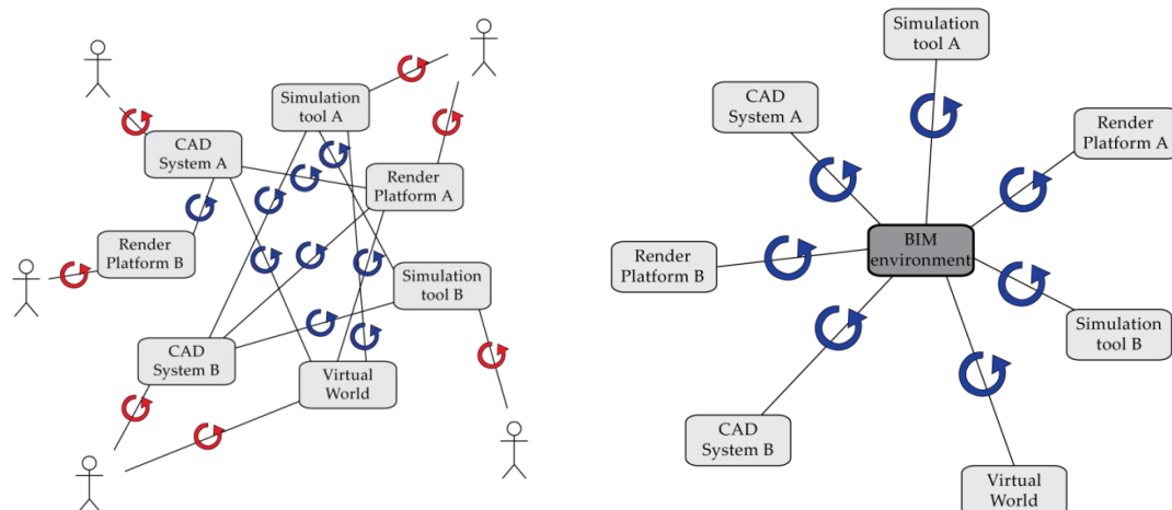
Figure 1: When sharing information 'in the wild' (left), end users need to manually compare new information with information that they manage. In a centralised model strategy (right), on the other hand, information is stored in one central location, and other applications refer to that information only and store to that central model only.
