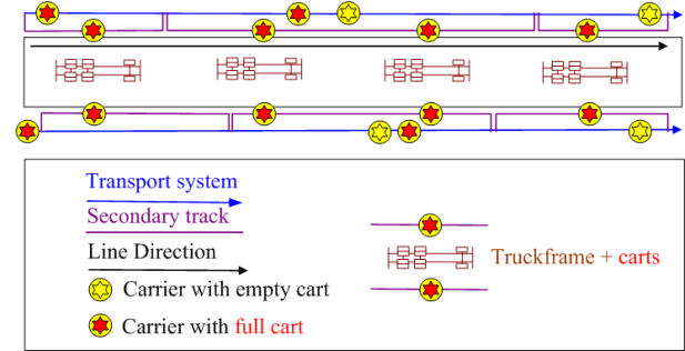
Figure 2: Dropoff Strategy 'Carrier Runs Along with the Line'
