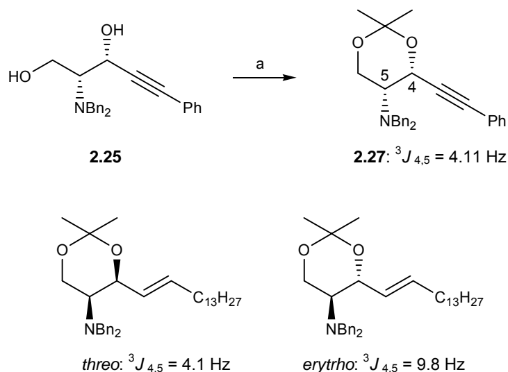
Scheme 7.6: Synthesis of dioxolane 2.27 and comparison of ^1\text{H} NMR data with previously reported compounds. 20b a) 2,2-dimethoxypropane/DMF (1:1), PPTS, RT, 2 h (85%).
