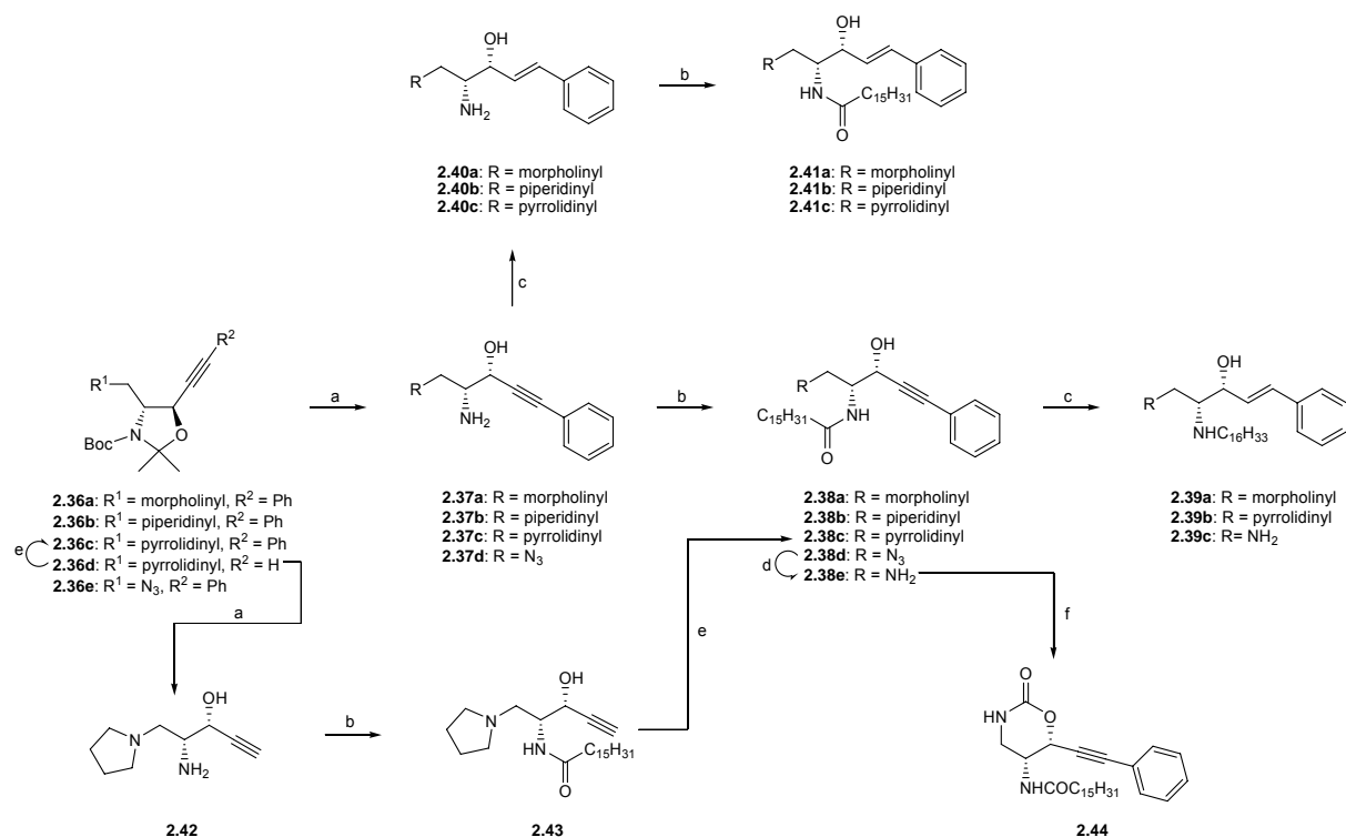
Scheme 2. Conditions: a) 3N HCl, MeOH, 50°C, 12 h; b) p -nitrophenylpalmitate, HOBT, pyridine, 50°C, 48 h; c) Red-Al, Et 2 O, -78°C to RT, overnight; d) PPh 3 , THF, RT for 30' then H 2 O, RT, 48 h; e) PdCl 2 (PPh 3 ) 2 , iodobenzene, piperidine, 70°C, overnight; f) triphosgene, TEA, CH 2 Cl 2 , 0°C to RT, 1h.
