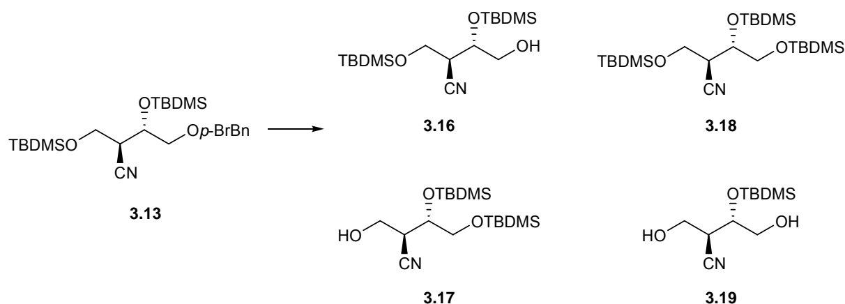
Scheme 11.5: Pd/C, H 2 , EtOH, RT, 4 h ( 3.16 + 3.17 : 32%; 3.18 : 10%; 3.19 , 50%)
