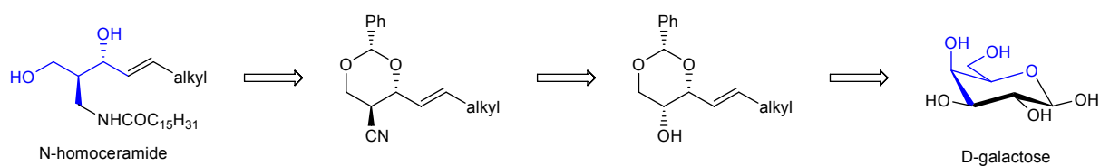
Figure 10.1: Retrosynthetic scheme for the synthesis of N-homoceramides starting from D-galactose. The sphingoid backbone is depicted in blue.
