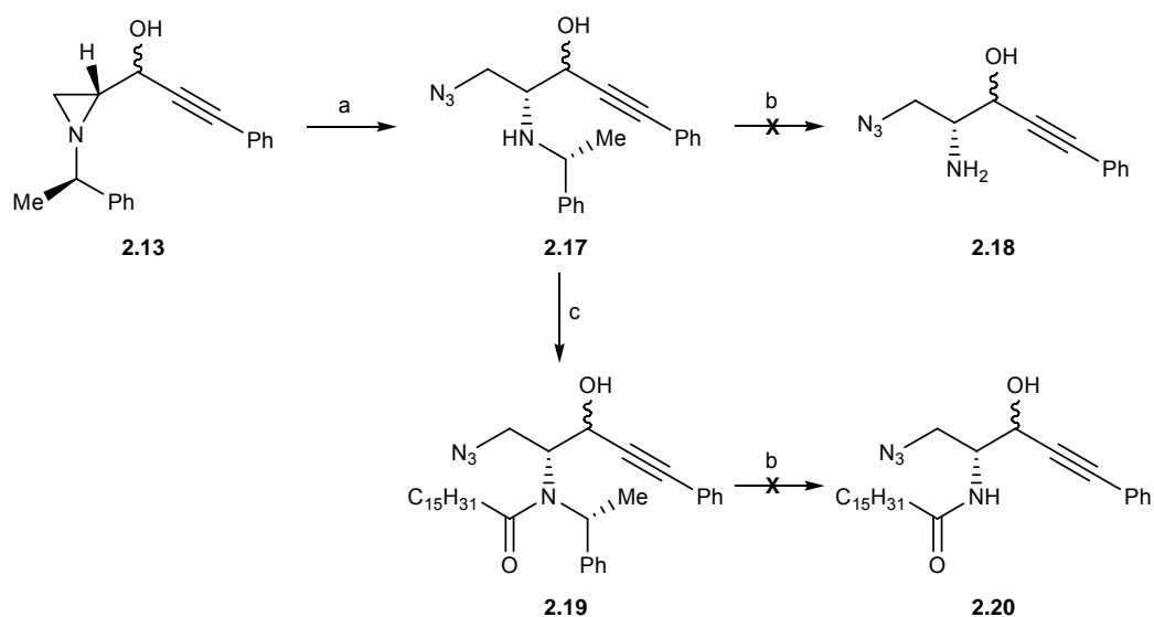
Scheme 7.3: a) \text{TMSN}_3 , \text{CH}_2\text{Cl}_2 , RT, 16 h (100%); b) see Table 7.2; c) palmitoyl chloride, DIPEA, \text{CH}_2\text{Cl}_2 , 0^\circ\text{C} to RT, overnight (78%).
