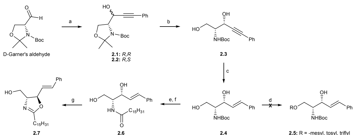
Scheme 6.1: a) lithium phenylacetylide, ZnBr 2 , Et 2 O, -78°C ( 2.1 : 44%; 2.1 + 2.2 : 28%); b) p -TsOH, MeOH, RT, 36 h (70%); c) Red-Al, Et 2 O, -78°C to RT, overnight (88%); d) see Table 6.1 ; e) 1N HCl:dioxane (1:1), reflux, 30' (72% crude yield); f) 50% NaOAc:THF (1:1), palmitoyl chloride, RT, 2 h, (58%); g) MsCl, TEA, CH 2 Cl 2 , 0°C to rt, 16 h (38%).
