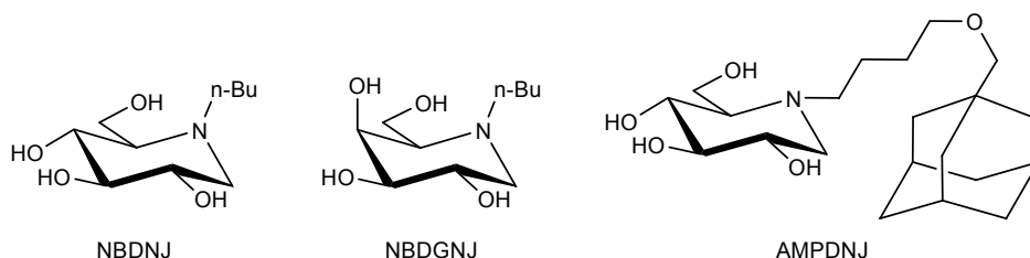
Figure 1.10: Structures of known inhibitors of glucosylceramide synthase
