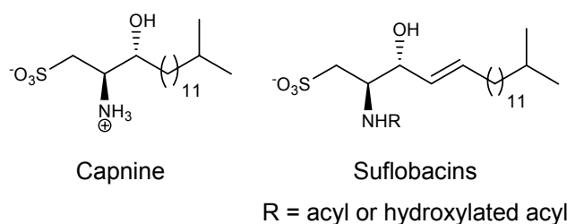
Figure 1.5: General structure of capnines and sulfobacins.
