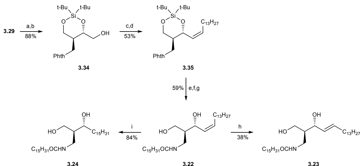
Scheme 3. Conditions: a) see Scheme 2 (100%); b) N -ethoxycarbonyl phthalimide, Hünig's base, THF, 75°C, 2 h (88%); c) Dess-Martin periodinane, \text{CH}_2\text{Cl}_2 , 0°C to RT, 3.5 h; d) PhLi, tetradecylphosphonium bromide, LiBr, \text{Et}_2\text{O} , THF, -78°C to RT, 5.5 h (53% from 3.34 ); e) hydrazine, EtOH, 55°C, 3 h (100% crude); f) palmitoylchloride, Hünig's base, \text{CH}_2\text{Cl}_2 , 0°C to RT, 1 h (65% from 3.35 ); g) TBAF, THF, RT, 3 h (91%); h) diphenyldisulfide, hv, cyclohexane/dioxane (3:1), RT, 4 h (38%); i) Pd/C, EtOAc, RT, 48 h (84%).
