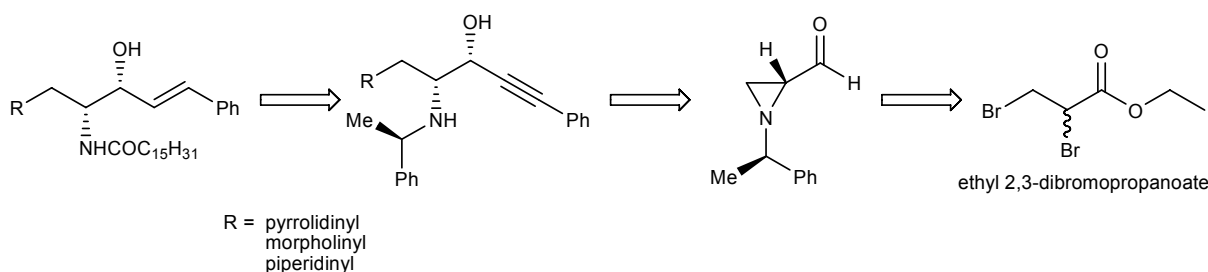
Figure 7.1: Retrosynthesis.
