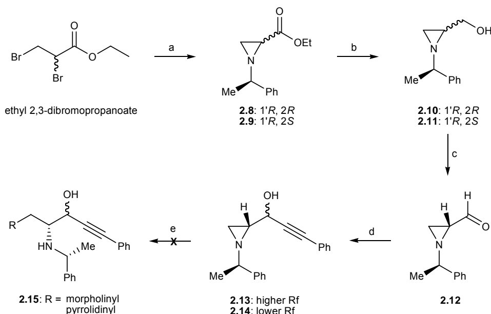
Scheme 7.1: a) R -(+)- \alpha -methylbenzylamine, TEA, 0°C to reflux, 3 h ( 2.8 : 19%; 2.9 : 17%; 2.8 + 2.9 : 60 %); b) LiAlH 4 , THF, 0°C to RT, overnight ( 2.10 : 97%; 2.11 : 95%); c) oxalylchloride, DMSO, TEA, CH 2 Cl 2 , -78°C to 0°C, 2.5 h (72%); d) lithium phenylacetylide, LiCl, THF, -78°C to RT, overnight ( 2.13 : 57%, 2.14 : 10%, 2.13 + 2.14 : 17%); e) see text.
