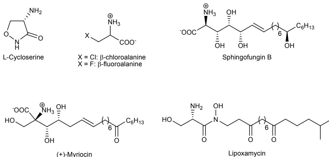
Figure 1.7: Known inhibitors of serine palmitoyltransferase.
