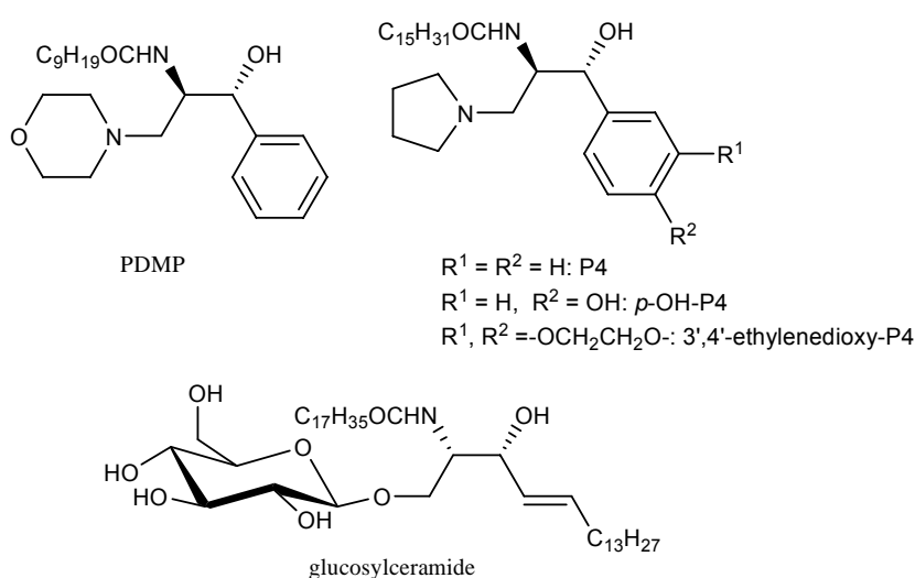
Figure 1.9: Structures of GlcCer, PDMP and PDMP analogues.
