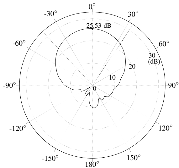
Fig. 5. Radiation pattern of the active wearable antenna at 1.6 GHz in the xz -plane
