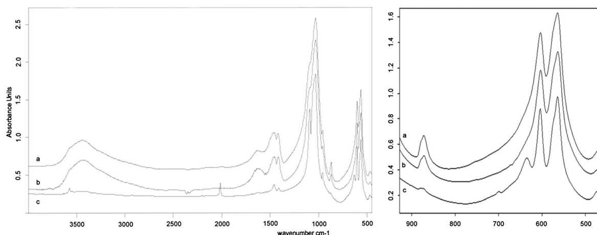
Figure 5. FTIR spectra of three bones of the same lime burial context at Son Matge rock shelter: a- brown bone (sample 9); b- black bone (sample 8); c- white bone (sample 7). Wavenumber \text{cm}^{-1} versus absorbance units.
