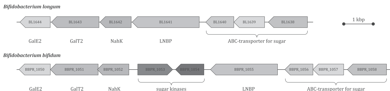
FIG 1 Schematic representation of the GNB/LNB gene cluster in B. longum NCC2705 (gene BL1638 to BL1644) and B. bifidum PRL2010 (gene BBPR_1050 to BBPR_1058). Two sugar kinases interrupt the GNB/LNB pathway of B. bifidum , and it is not organized as in the lnpABCD operon (BL1641 to BL1644) of B. longum .
