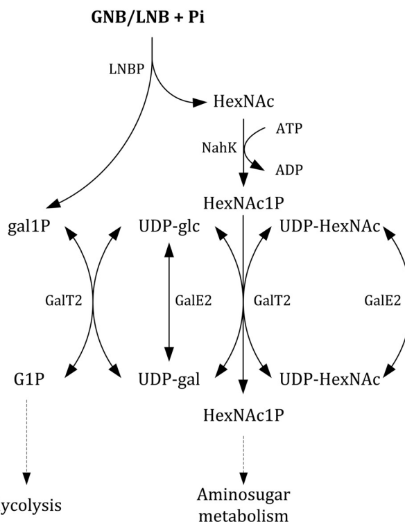
FIG 2 Overview of the Leloir pathway (A) and GNB/LNB pathway (B) in Bifidobacterium bifidum . LNBp, NahK, GalT2, and GalE2 are encoded in the same gene cluster (4). In contrast, the classic Leloir pathway (A) is encoded by scattered genes, and evidence is lacking for the existence of metabolic crossover between both pathways. Gene locus tags of the corresponding enzymes are listed in Table 1.
