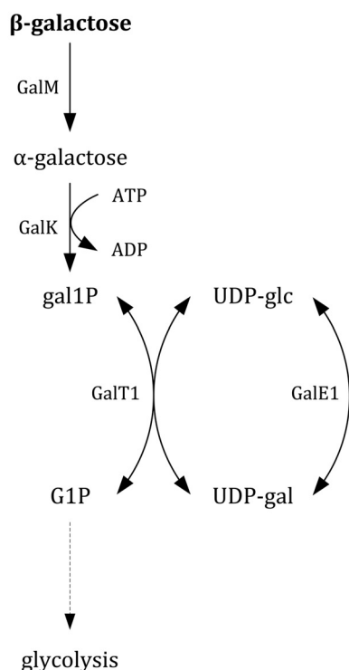
FIG 2 Overview of the Leloir pathway (A) and GNB/LNB pathway (B) in Bifidobacterium bifidum . LNBp, NahK, GalT2, and GalE2 are encoded in the same gene cluster (4). In contrast, the classic Leloir pathway (A) is encoded by scattered genes, and evidence is lacking for the existence of metabolic crossover between both pathways. Gene locus tags of the corresponding enzymes are listed in Table 1.
