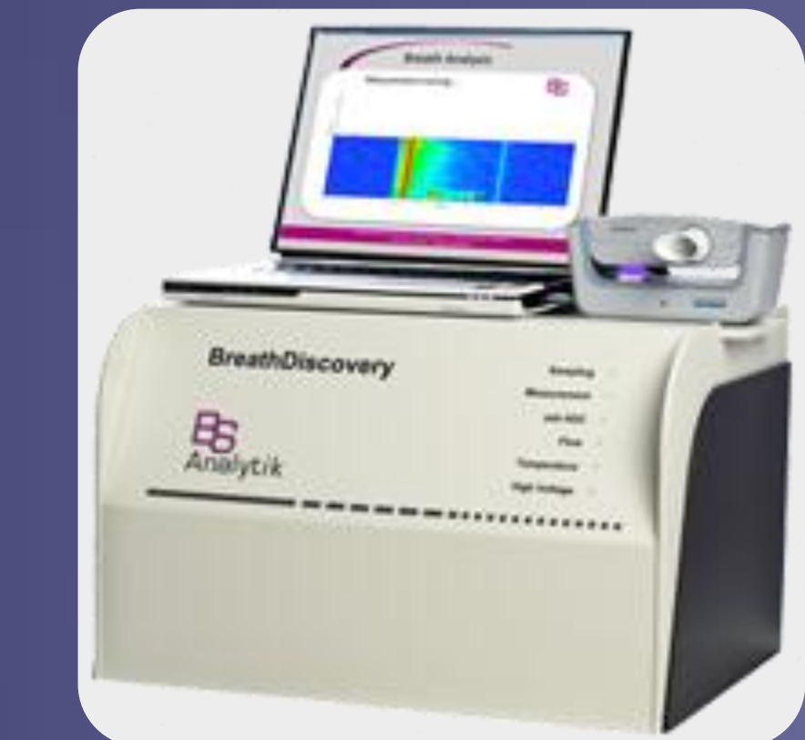
Figure 2: The MCC/IMS device (BioScout) with sampling unit (SpiroScout).
