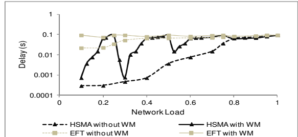
Fig. 5: Delay with and without WM in HSMA and EFT
