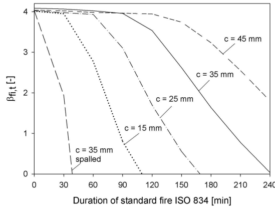
Figure 1: Reliability \beta_{fi,t} as a function of the ISO 834 duration, for different values of the concrete cover c
