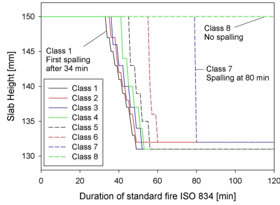
Figure 2: Spalling behavior for different classes of f_{ct,20^{\circ}\text{C}} as a function of the fire exposure time
