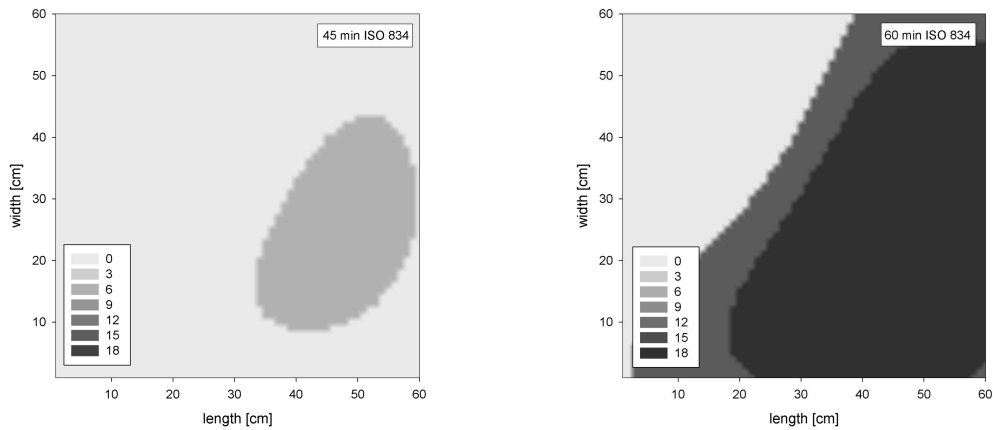
Figure 4: Example 2 of the spatial occurrence of spalling for a concrete slab with mean f_{ct,20^{\circ}C} of class 6 (3.1 MPa) for different ISO 834 durations – second realization of the random field
