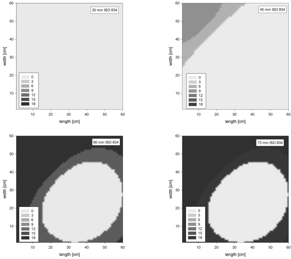
Figure 3: Example 1 of the spatial occurrence of spalling for a concrete slab with mean f_{ct,20^{\circ}C} of class 6 (3.1 MPa) for different ISO 834 durations – first realization of the random field
