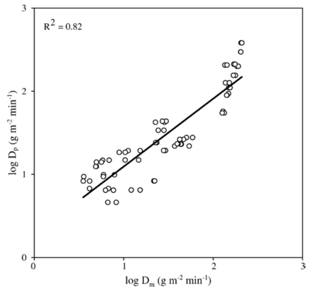
Fig. 8. Scatter plot of measured ( D_m ) versus predicted ( D_p ) sand detachment rates by a log-linear regression.
