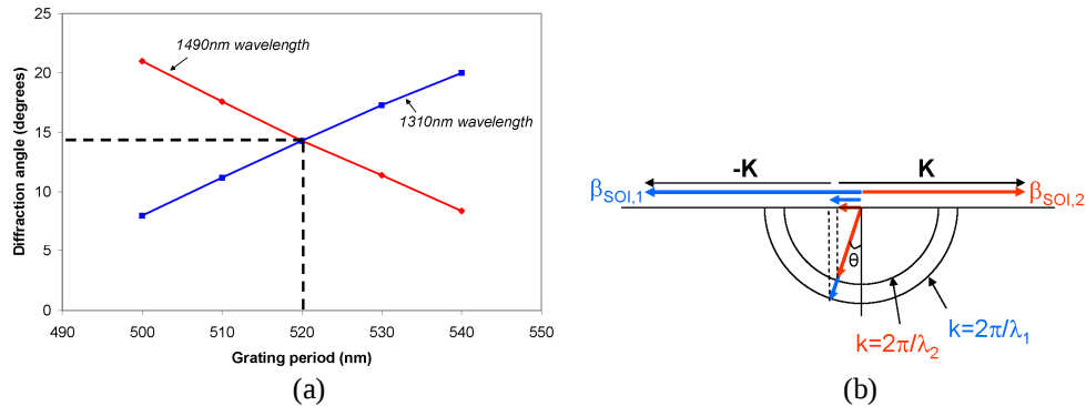
Fig. 2. Diffraction angle of light with a wavelength of 1310nm (1490nm) exciting the grating from the left hand side (right hand side). The intersection of both curves determines the working point for duplexer operation (a) and the wavevector diagram for the duplexer configuration (b)
