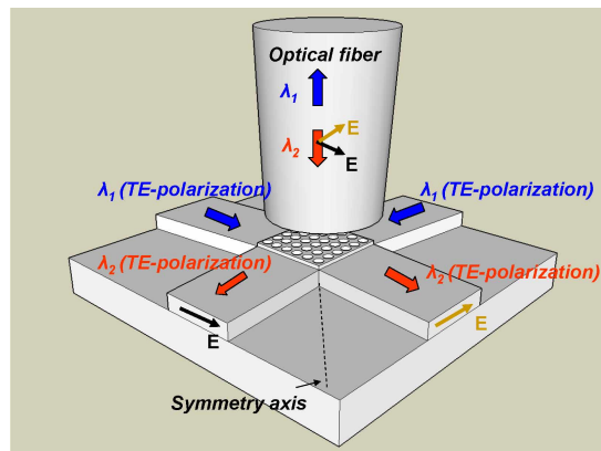
Fig. 7. Layout of the grating duplexer structure for polarization diversity operation
