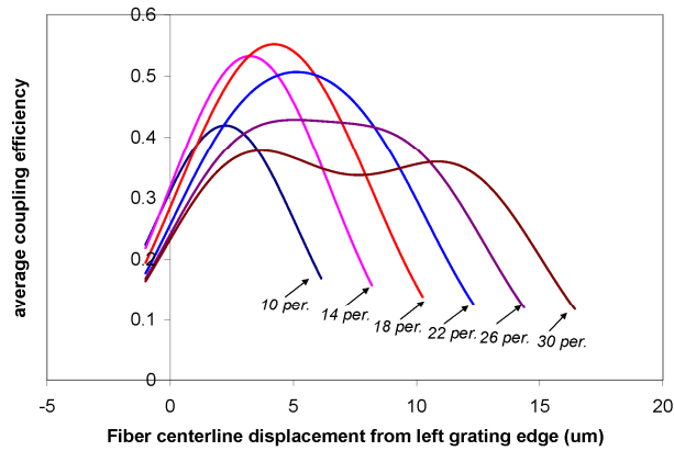
Fig. 3. Average fiber coupling efficiency of both wavelength channels as a function of the number of grating periods and the position of the optical fiber
