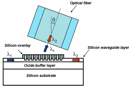
Fig. 1. Proposed design of an ultra-compact wavelength duplexer based on diffractive fiber-to-waveguide grating couplers
