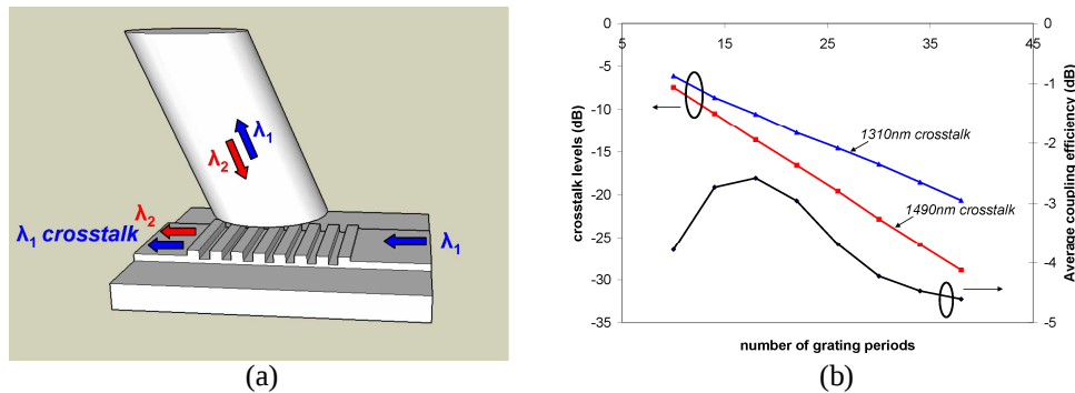
Fig. 6. Origin of crosstalk when using this duplexer structure in transceiver configuration (a) and the influence of the grating length on crosstalk and average fiber coupling efficiency (b)
