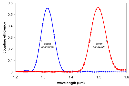
Fig. 4. Coupling efficiency spectrum for both wavelength channels for the optimized duplexer grating
