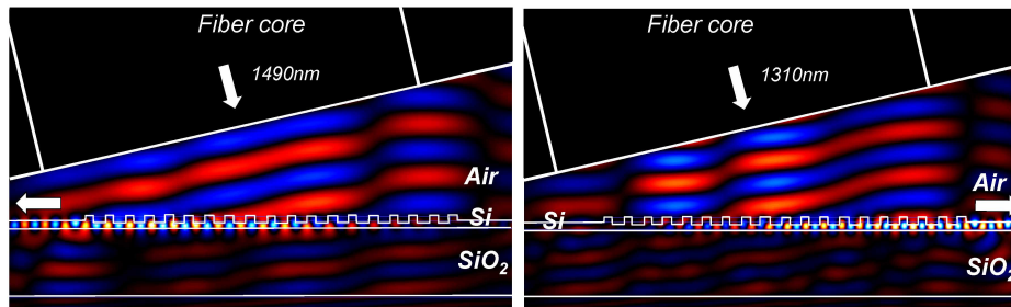
Fig. 5. Electric field plot of the duplexer grating structure when illuminated from an optical fiber for both wavelength channels, illustrating the duplexing behavior.
