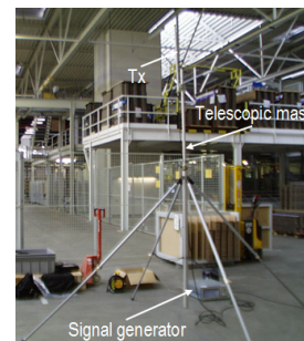
Fig. 1. Transmitter configuration
