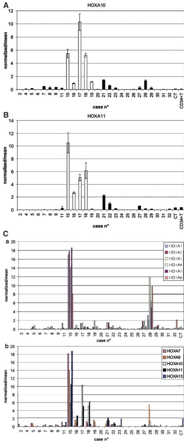
Figure 4 (A) Geometric averages of normalized expression of HOXA10 in inv(7) positive T-ALL cases (white boxes), inv(7) negative T-ALL cases (black boxes), total child thymocytes (CT) and CD34+ sorted stem cells (CD34+T). (B) Geometric averages of normalized expression of HOXA11 in inv(7) positive T-ALL cases (white boxes), inv(7) negative T-ALL cases (black boxes), total child thymocytes (CT) and CD34+ sorted stem cells (CD34+T). (C (a and b)) Global overview of normalized expression of all class I HOX genes tested in inv(7) positive T-ALLs (cases no. 15–19), inv(7) negative T-ALLs (cases no. 2–11 and no. 20–32) and total child thymocytes (CT).
