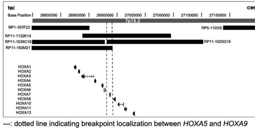
Figure 2 Base position of HOXA flanking (RP1-167F23 telomeric and RP5-110315 centromeric) and HOXA covering clones (RP11-1132K14, RP11-1036C18, RP11-163M21 and RP11-1025G19), according to UCSC Genome Browser May 2004 Freeze.
