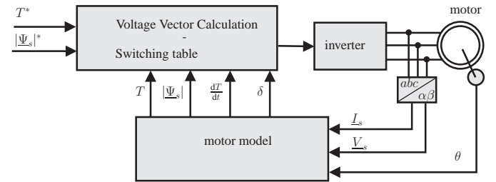
Fig. 4: Predictive DTC
