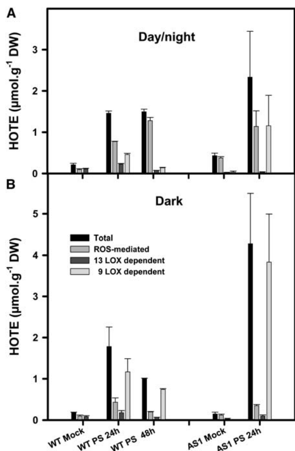
Figure 6. Comparison of lipid peroxidation in P. syringae pv syringae -infected leaves of wild-type (WT) and catalase-deficient transgenic (Cat1AS) plants. Leaves from plants grown at LL (100 \mu\text{mol m}^{-2} \text{s}^{-1} fluence rate; day/night, 14/10 h) were infiltrated with P. syringae pv syringae ( 5 \times 10^7 cfu \text{mL}^{-1} in 10 mM \text{MgCl}_2 ) and incubated in (A) HL (350 \mu\text{mol m}^{-2} \text{s}^{-1} fluence rate; day/night, 14/10 h) or (B) the dark. The upstream oxylipin profile of Pseudomonas -inoculated leaves was determined after 24 h of incubation for wild type (WT PS 24 h) and Cat1AS (AS1 PS 24 h) plants and also after 48 h for wild-type (WT PS 48 h) plants; \text{MgCl}_2 -inoculated leaves were included as controls and analyzed after 24 h of incubation (WT Mock and AS1 Mock). See Figure 3 for lipid peroxidation characterization. Results expressed as mean \pm SD ( n = 3 ).
