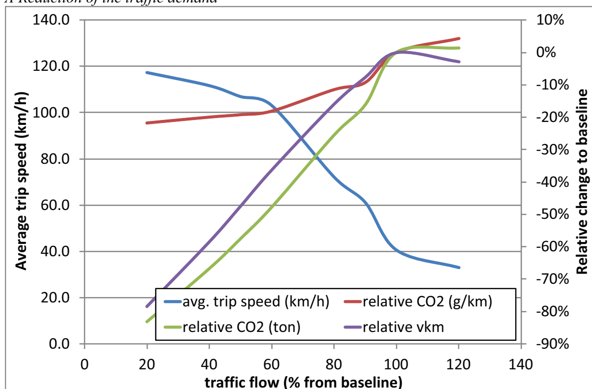
Figure 5 - Average trip speed, emissions of CO 2 (total and per km) and vehicle kilometres on the E313 for different traffic demands.
