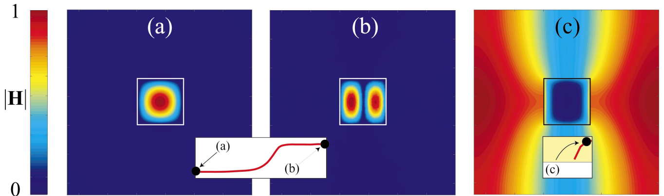
FIG. 5. (Color) Magnetic field profiles ( |\mathbf{H}| ) of the TE-polarized states at three representative points on the band structure diagram in Fig. 4. (a) [\omega=0.3(2\pi c/a), k=\Gamma] and (b) [\omega=0.355(2\pi c/a), k=X] show the field localization at the band edges of the second band. (c) [\omega=0.44(2\pi c/a), k=0.475(2\pi/a)] shows the metallic profile above \omega_T .
