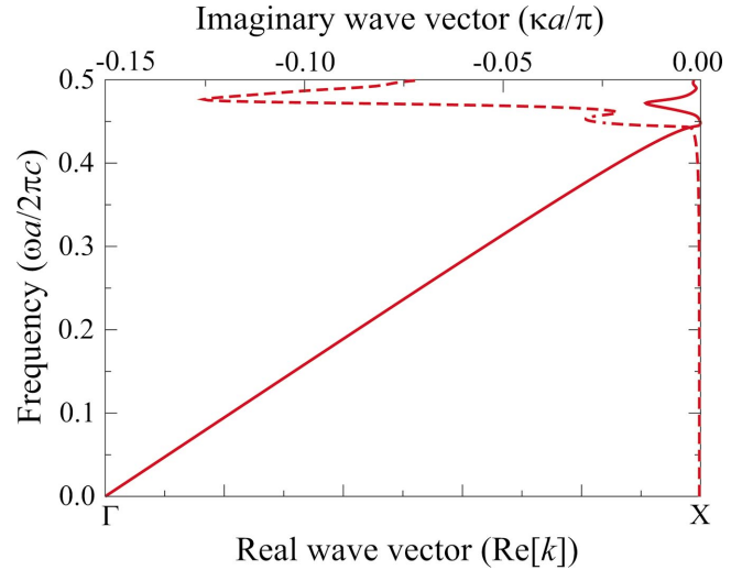
FIG. 8. (Color) Real (solid) and imaginary (dashed) wave-vector components from a real- \omega simulation of the TE bands of a crystal of square SiC rods with s/a=0.25 , \epsilon_\infty=6.7 , \omega_T=0.5(2\pi c/a) , \omega_L=0.6(2\pi c/a) , and \gamma=0.01(2\pi c/a) . Note that the modes remain close to the edge of the Brillouin zone at frequencies near \omega_T , unlike the lossless crystal which has flat bands extending from \Gamma to X .
