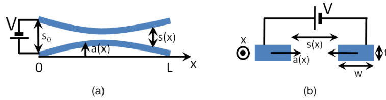
Fig. 3. Mathematical description of the slot waveguide based phase modulator: (a) top view, (b) cross sectional view.
