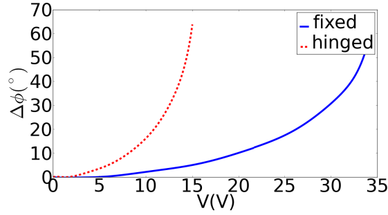
Fig. 5. Theoretically predicted phase change as a function of applied voltage across the slot with L = 5.8 \mu\text{m} for fixed and hinged boundary conditions.
