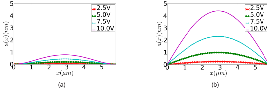
Fig. 4. Beam excursion of one of the beams as a function of x for different applied voltages: (a) fixed boundary conditions, (b) hinged boundary conditions.
