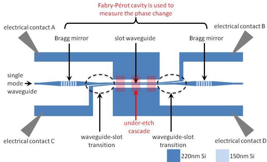
Fig. 8. Schematic layout of the NEMS based phase modulator.
