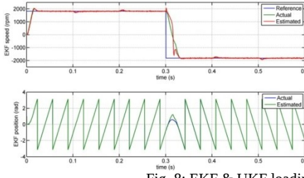
Fig. 8: EKF & UKF loading & un-loading performance
