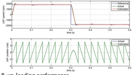
Fig. 8: EKF & UKF loading & un-loading performance
