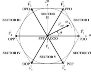
Fig. 2: Diagram of voltage space vector
