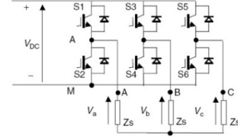
Fig. 1: Three phase, two level inverter
