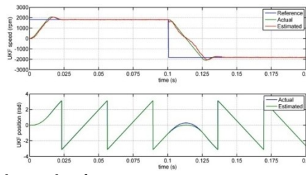
Fig. 6: EKF & UKF speed reversal performance
