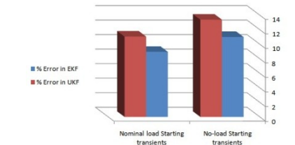
Fig. 10: EKF & UKF loading & un-loading error
