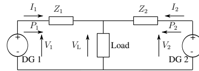
Fig. 1. Two DG units in resistive network
