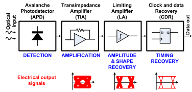
Figure 2. OLT's 3R (Recovery) BM-Rx
