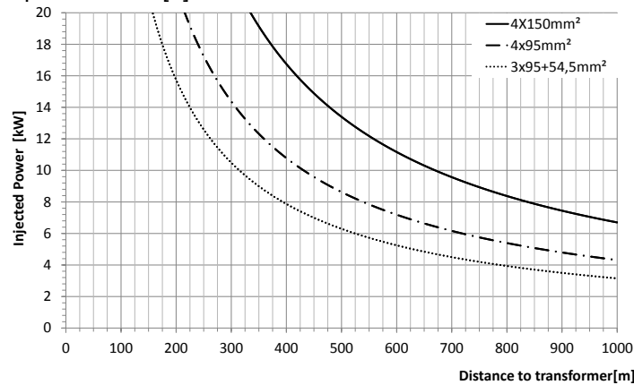
Figure 1: hosting capacity for 10% over voltage limit for different grid types.
