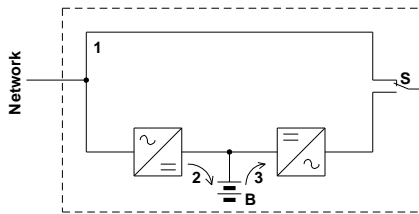
Figure 5: passive standby UPS
