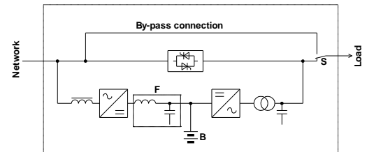
Figure 7: double conversion UPS
