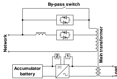
Figure 6: line interactive UPS
