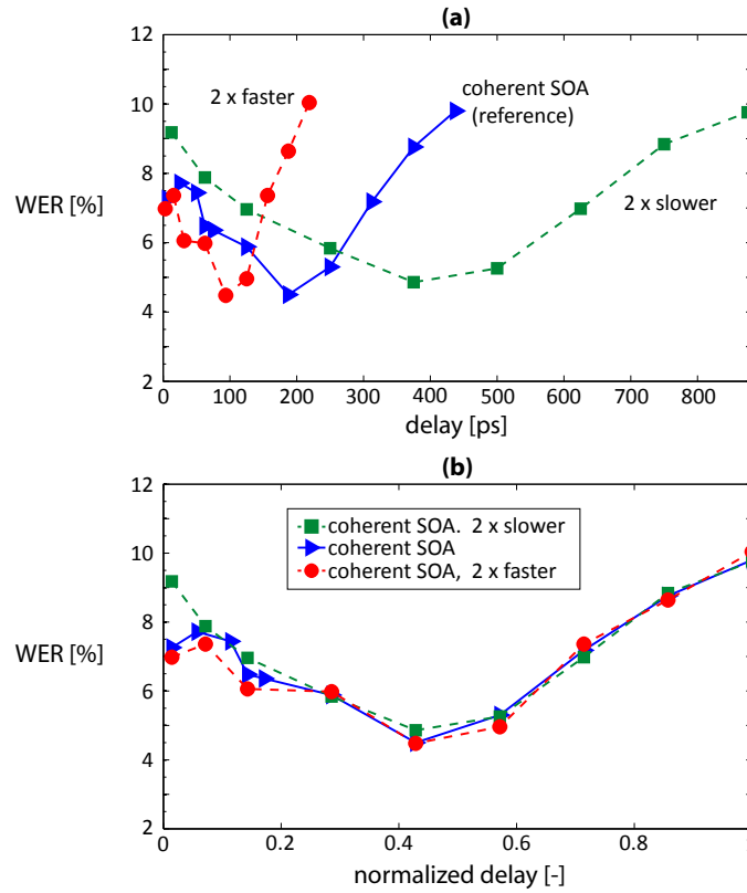
Figure 2: (a) Results for different speeds of the input signals fed into a coherent swirl SOA reservoir, (b) the same results but plotted on top of each other by changing the X-axis of the different curves the same way as their input rate.
