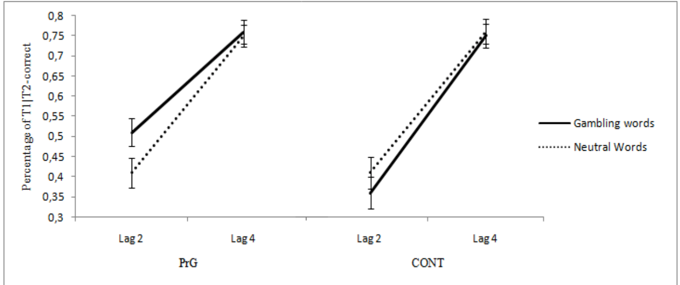
Figure 1. Percentage of T1|T2-correct for CONT and PrG with gambling-related and neutral stimuli.
