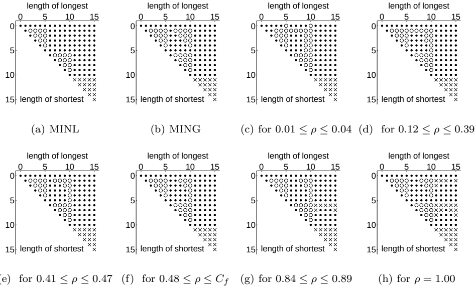
Figure 2: Each CDS algorithm can be represented by an action table, with an action for each combination of longest horizon (x-axis) and shortest horizon (y-axis). The actions \{1 (join shortest), 2 (join longest), 3 (drop) \} are indicated by \{\bullet, \circ, \times\} , respectively. A degenerate buffer is assumed, with N = 2 , \mathcal{A} = \{0, 5, 10\} , a Bernoulli arrival process, and B fixed to 6. The CDS algorithms (c-e) are optimal in the indicated interval, regardless of whether preventive drop is considered or not. The CDS algorithm (f) is optimal for 0.48 \leq \rho \leq C_f , with C_f = 0.65 if preventive drop is considered, and C_f = 1.00 if no preventive drop is allowed. The CDS algorithms (g-h) are optimal in the indicated interval only if preventive drop is allowed.
