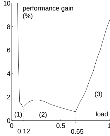
Figure 5: When compared to MING, a load-dependent mechanism yields much better loss performance when the load is low (zone (1) in the figure). For intermediary load ( 0.12 \leq \rho \leq 0.65 , zone (2)), loss reduction is limited to 1–2 %, whereas for high load (zone (3)), the performance gain is again larger.
