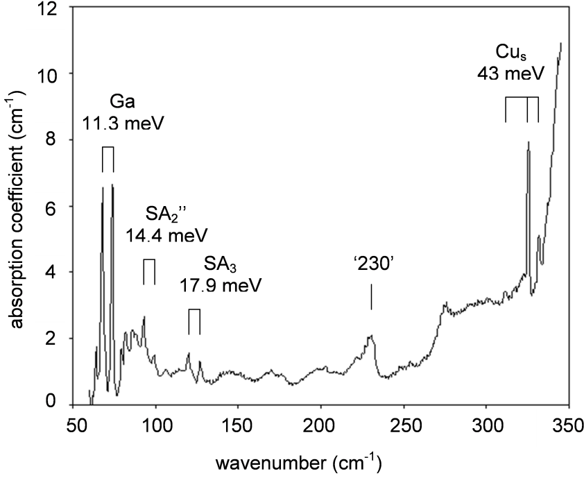
Figure 2: FTIR spectrum of a sample quenched from 825^\circ\text{C} in Santovac 5 oil. Beside the acceptor series from substitutional Cu and from the Ga dopant, also absorption lines are seen from semi-shallow quenched-in acceptors [27].
