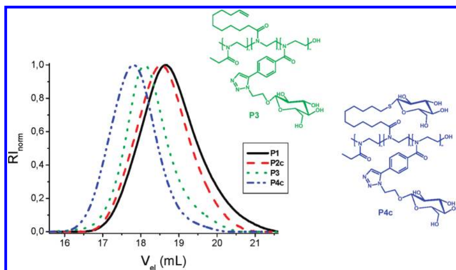
Figure 5. SEC traces of the initially obtained copolymer ( P1 ) and the product of the thiol–ene reaction with \text{GlcAc}_4\text{SH} ( P2c ) and their deprotected products ( P3 , P4c ) (DMA/2.1 g L -1 LiCl; PS standard).
