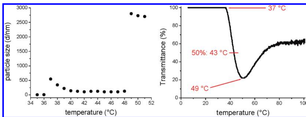
Figure 7. Temperature dependence of the particle size determined by DLS measurements (left) and transmittance (right) of P4c (1 mg · mL -1 ; PBS solution).
