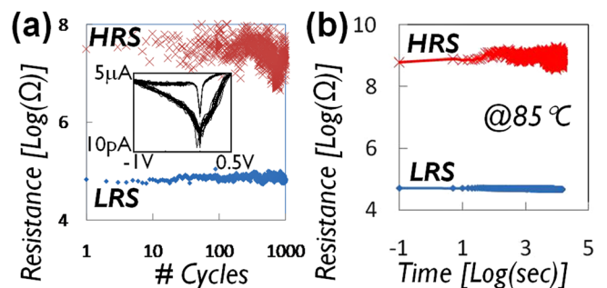
FIG. 4. (Color online) (a) HRS and LRS resistance control observed over 10^3 I - V cycles using I_{COMP} = 5 \mu\text{A} (inset shows 30 consecutive I - V cycles); (b) HRS and LRS resistance monitoring at 85^\circ\text{C} using constant bias voltage of 20\text{mV} .
