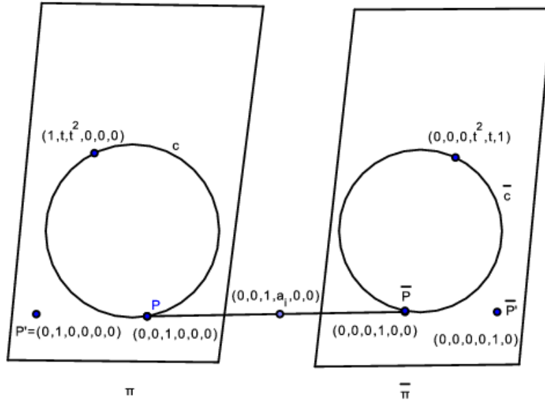
Figure 6. A 2-saturating set in PG(5, q)
