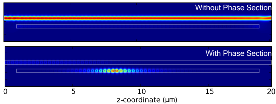
Figure 3: Intensity profile of EBR and CER at Bragg wavelength ( \lambda = 1.591 \mu\text{m} )
