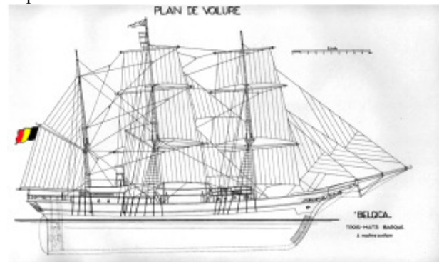
Figure 2 Sailplan of the original Belgica . [1]
