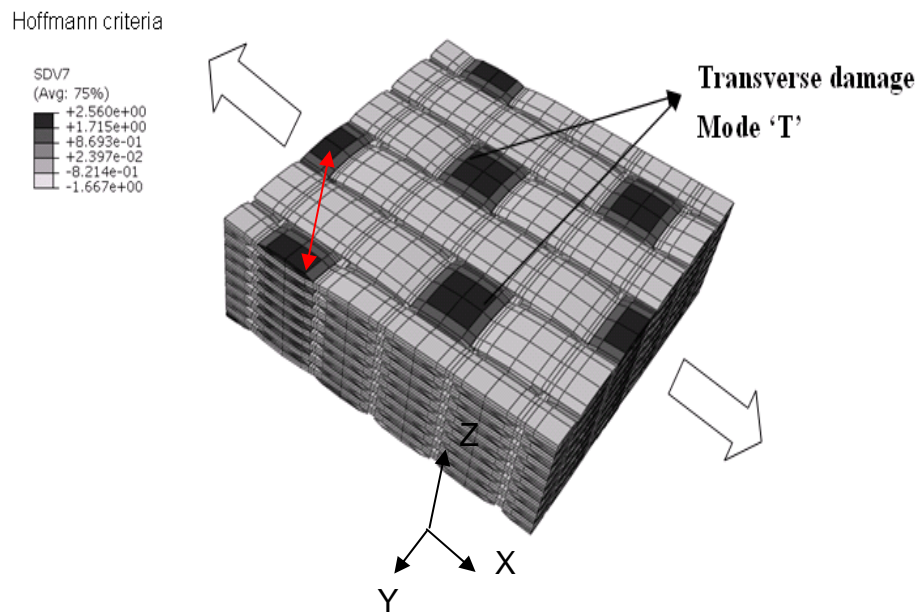
Figure 3. 8 unit cell stack FE analysis : a) Transverse stress distribution on the weft yarn; b) Transverse damage locations on the weft yarn at the yarn crimp location <0.44\% with the 8 unit cell in-phase stack, in-plane PBC.
