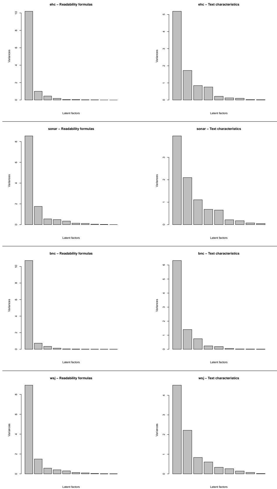
Figure 1: For each corpus, two bar charts showing the explained variances of principal components. For the charts on the left, the principal components are found by comparing the 12 readability formulas put forward in table 2. For those on the right, the variables used in the readability formulas were compared.
