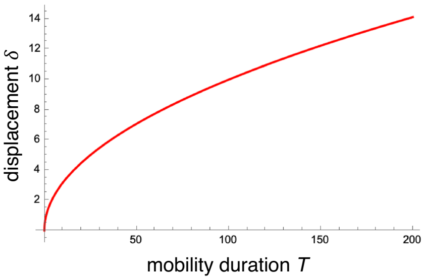
Fig. 4 The relationship between the most probable distance traveled (mean square displacement) and the time spent engaged in motion given unbiased Brownian motion
