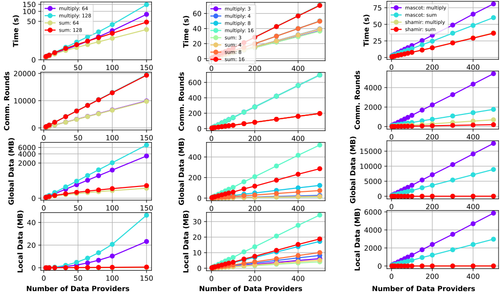
(a) Direct-decentralised MPC. Time and global data are in cubic-root scale . Legend shows the computation & array size.
