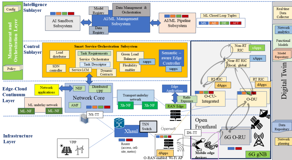
Figure 1: Proposed Unified Architecture of UNITY-6G
