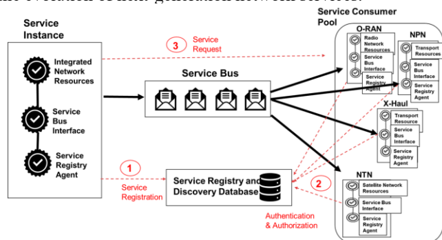
Figure 3: Providing UNITY-6G integrated services (belonging to different domains)
