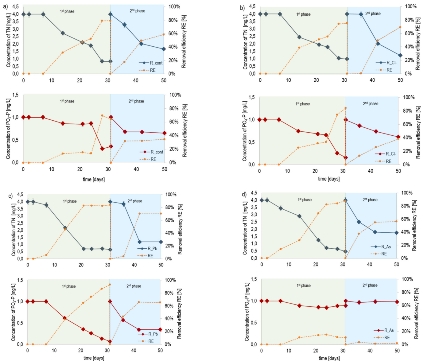
Fig. 1. Changes in TN and \text{PO}_4\text{-P} concentrations (uncertainty intervals \pm 10\% ) and removal efficiencies in a) R_{\text{cont}} , b) R_{\text{Cl}} , c) R_{\text{Pb}} , and d) R_{\text{As}} treatments during two phases of the experiment (1st and 2nd phases). Control reactor ( R_{\text{cont}} ), chloride treated reactor ( R_{\text{Cl}} ), lead treated reactor ( R_{\text{Pb}} ), and arsenic treated reactor ( R_{\text{As}} ), removal efficiency (RE), total nitrogen (TN), orthophosphate phosphorus ( \text{PO}_4\text{-P} ).
