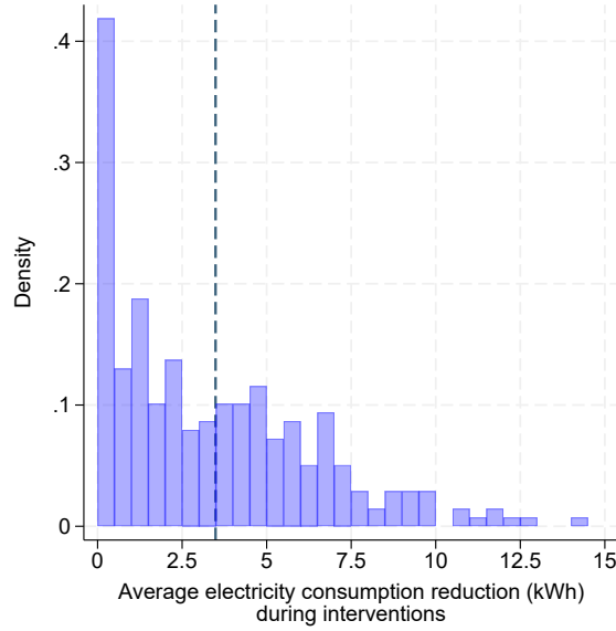
Figure 3: Histogram of the average decrease in electricity consumption (in kWh) during each intervention, computed using the average daily heat pump consumption profile as the counterfactual (defined in eq. (3)). The dotted line indicates the mean energy saved. The histogram is truncated at 15 kWh to exclude outliers.
