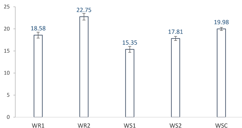
Figure 11. Average carbonation depth. The error bars represent the standard error of the average.
