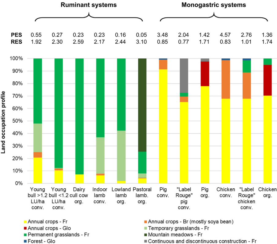
Fig. 2. Simplified land occupation (LO) profiles of the animal-production systems studied (m 2 yr required to produce 1 kg of human-edible animal protein). PES: score of provisioning ecosystem service; RES: score of regulating & maintenance ecosystem service. Maximum score = 5. LU: livestock unit; Fr: France; Br: Brazil; Glo: global; conv.: conventional; org.: organic.
