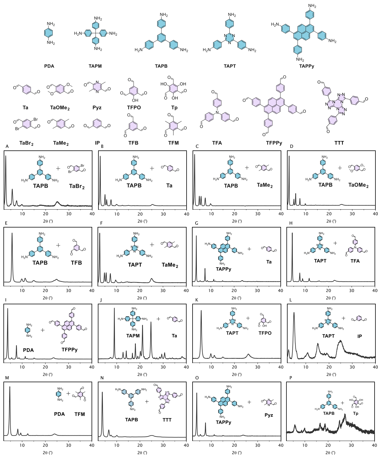
Figure 5. Overview of the different monomers and PXRD patterns of the 16 attempted COFs
