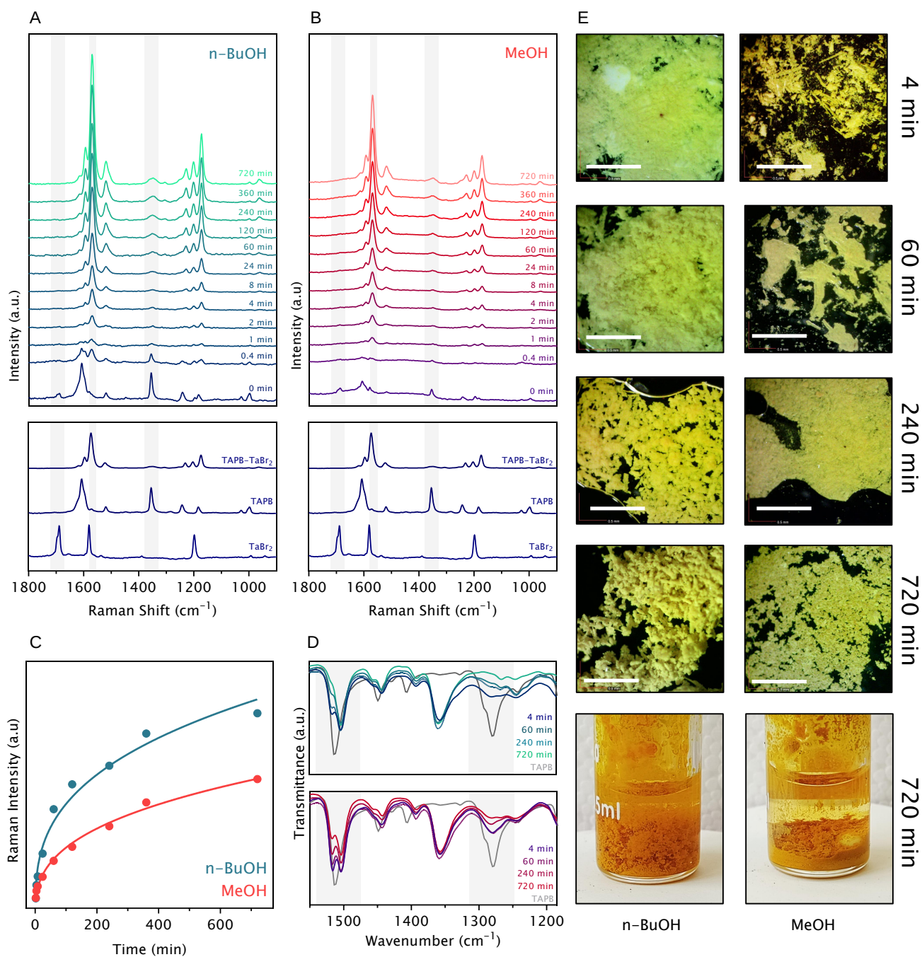
Figure 3. Evolution over time of the Raman spectrum of a mixture of TAPB and TaBr 2 in (A) n-butanol and (B) methanol; The intensity of the C=C stretch at 1570 cm -1 over time of the reaction mixture containing n-BuOH (teal) or methanol (red) (C); FTIR spectra of the washed and dried TAPB-TaBr 2 synthesised in reaction mixtures with n-butanol (top) or methanol (bottom) (D); Optical microscopy images and photographs of TAPB-TaBr 2 during synthesis in n-butanol (left) or methanol (right) at different points in time. The white bar is 1 mm. (E)
