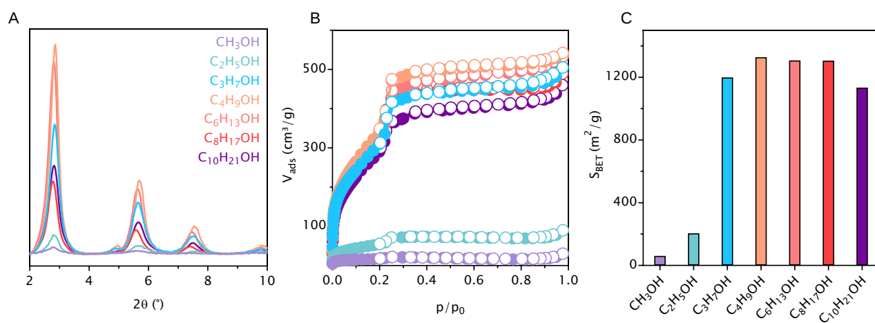
Figure 2. The PXRD patterns, N 2 -sorption isotherms, and calculated S_{BET} of TAPB-TaBr 2 synthesized using different alkyl alcohols
