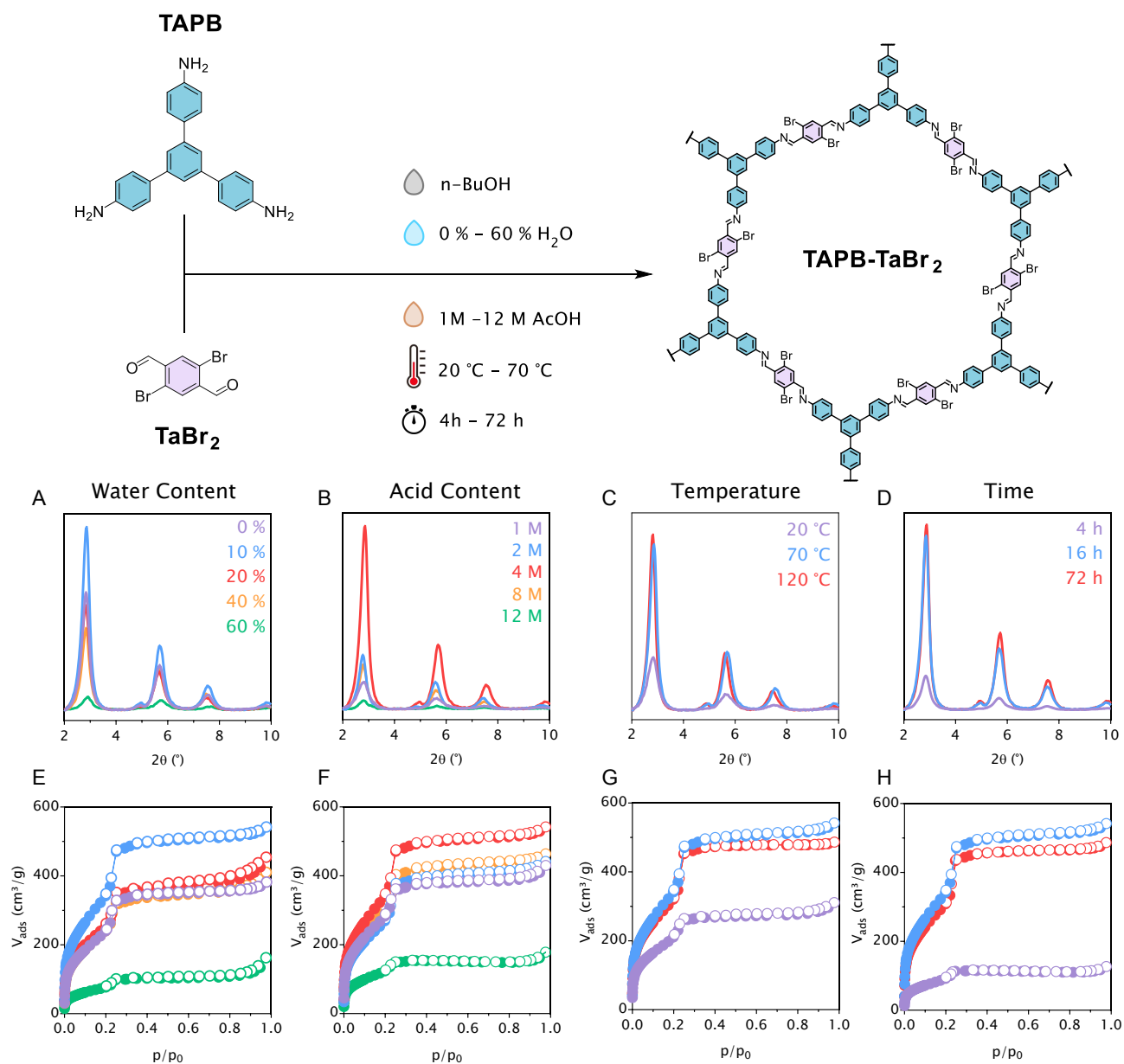
Figure 1. PXRD patterns and N 2 -sorption isotherms of TAPB-TaBr 2 COF synthesized in n-BuOH with variation of the water content (A,E), acetic acid content (B,F), reaction temperature (C,G) and time (D,H) from base parameters (10 v% H 2 O, 4 M AcOH, 16 h, 70 °C).
