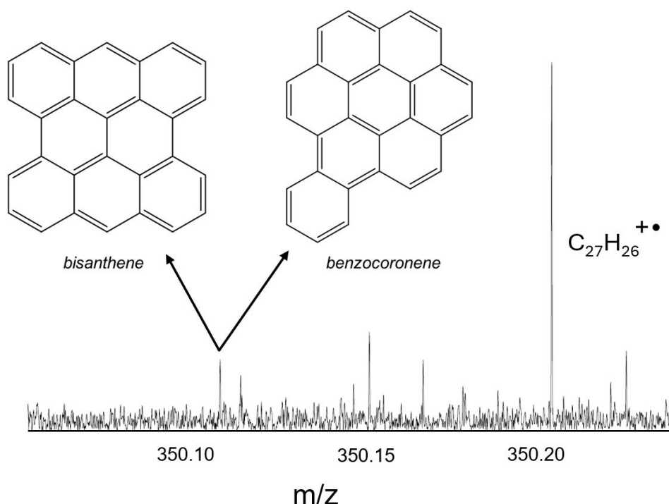
Figure 2. Molecular structures of bisanthene and benzocoronene, which correspond to molecular formulas assigned to mass spectral peaks detected by (+)APPI 21 Tesla FT-ICR MS in MPO pyrolysis oil.
