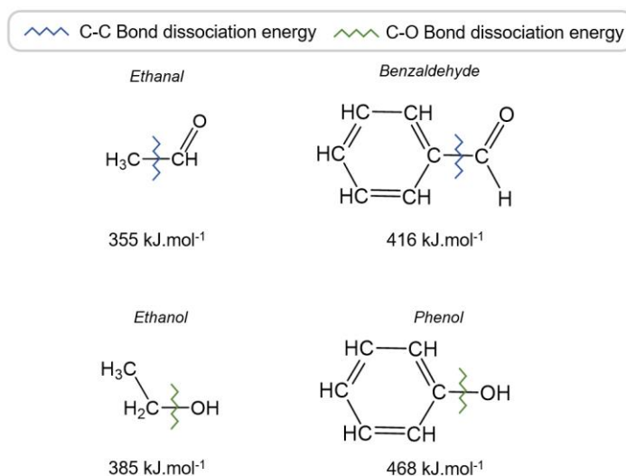
Figure 4. Bond dissociation energies of the C-C bond of ethanal and benzaldehyde and C-O bond of ethanol and phenol. Data obtained from 72, 73 .
