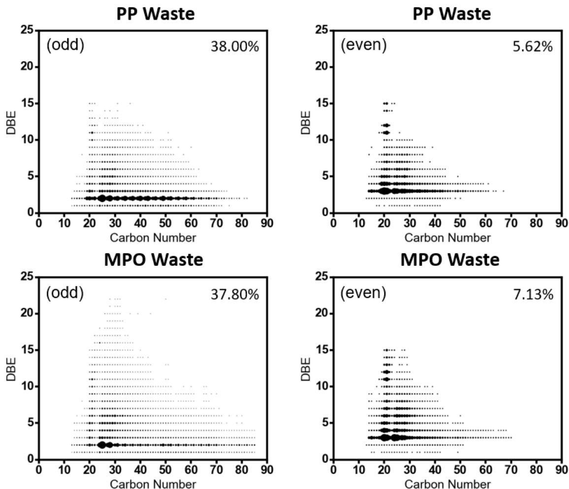
Figure 1. (+)APPI-mode DBE versus carbon number plots for hydrocarbons from the virgin LDPE, PE waste, PP waste and MPO waste. The area of the dots is proportional to the relative abundance of the respective molecular formula. Odd-electron ions (left) and even-electron-ions (right) are presented with the relative abundance of every class presented in the top right corner.
