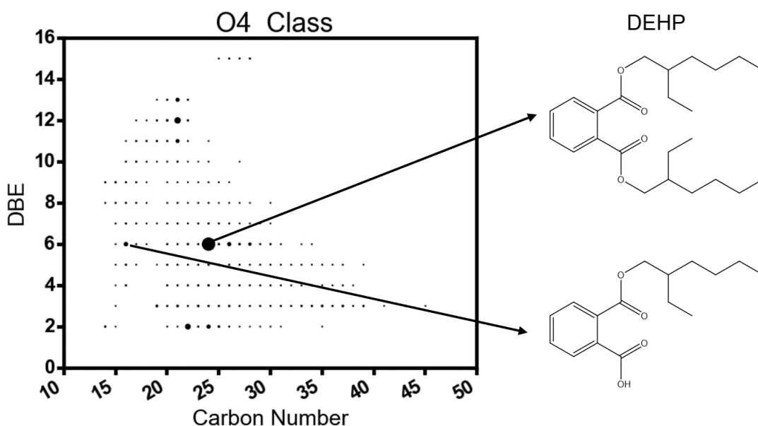
Figure 6. The DBE versus carbon number plot of even-ion O4 for waste PP pyrolysis oil by (+)APPI with (top) diethylhexyl phthalate (DEHP) and (bottom) 2-(((2-ethylhexyl)oxy)carbonyl)benzoic acid indicated
