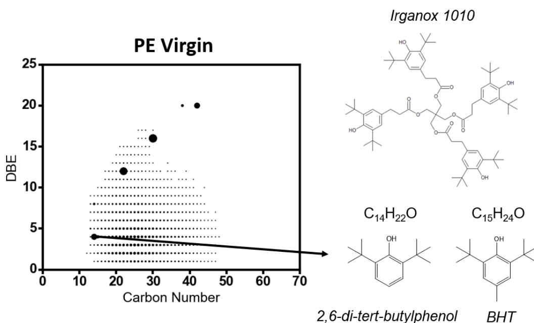
Figure 8. The molecular structures of 2,6-di-tert-butylphenol, butylated hydroxytoluene (BHT), and Irganox 1010
