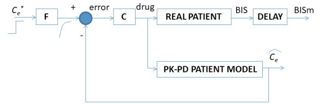
Fig. 8. Control scheme with patient model estimation.
