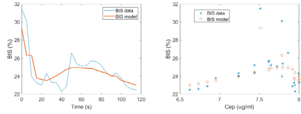
Fig. 7. Example of BIS data and BIS estimated during analgesic region (left) and corresponding reduced surface model identification (right) for Patient 24 from (Ionescu et al., 2024).
