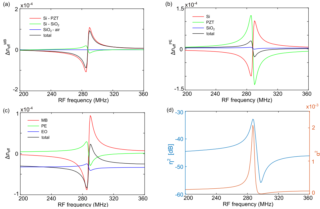
FIG. 11. Calculation of the index modulation from the simulated results: (a) \Delta n_{\text{eff}}^{\text{MB}} plot for different interfaces in the waveguide mode region, (b) \Delta n_{\text{eff}}^{\text{PE}} plot for different layers in the waveguide system, (c) \Delta n_{\text{eff}} contribution from different mechanisms, and (d) log and linear plot of the net phase modulation.
