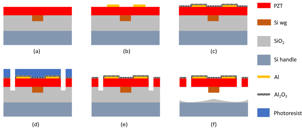
FIG. 3. Schematic diagram showing the process flow. (a) PZT deposition on planarized Si PIC, (b) fabrication of the Al electrodes, (c) ALD deposition of 50 nm \text{Al}_2\text{O}_3 and partial etching of \text{Al}_2\text{O}_3 film from the contact pads, (d) etching through \text{Al}_2\text{O}_3 /PZT layers to create etch windows, (e) removal of the photoresist mask followed by dehydration of the sample, and (f) HF vapor exposure to etch \text{SiO}_2 .
