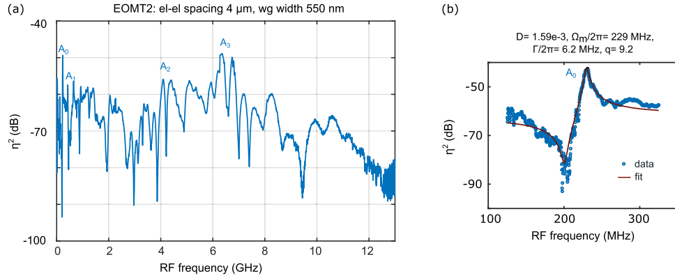
FIG. 7. (a) Modulation efficiency ( \eta^2 ) for EOMT2 driven with 14 dBm RF power. (b) Measurement data of the primary Fano resonance and fit with the Fano formula. Again, here the deviation between the data and the fit looks exaggerated at the lower values due to the logarithmic scale.
