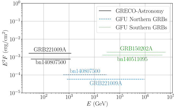
Figure 6. Limits on per-flavor time-integrated neutrino number flux, F(E) , times E^2 for six GRBs. Black lines show two GRBs studied with GRECO-Astronomy. One GRB is bn 140807500 (TW = 100 s), the most significant GRB identified in this work, and the other is GRB 221009A (TW = T_{90,GBM} ) (Abbasi et al. 2023a). Blue lines are for two northern sky GRBs, studied with tera electronvolt to peta electronvolt neutrinos, using the GFU (Gamma-ray Follow-Up) data set. These are, again, bn 140807500 (for TW = 100 s) (Abbasi et al. 2022b) and GRB 221009A (TW = T_{90,GBM} ) (Abbasi et al. 2023a). Green lines are for two southern sky bursts: GRB 150202A (TW = 2 days) and Fermi GRB bn 140511095 (TW = 2 days) (Abbasi et al. 2022b). The energy ranges shown correspond to the central 90% of neutrino energies that would contribute to an E^{-2} signal. The sensitivity of GRECO-Astronomy varies by a factor of \sim 2 as a function of decl. On the other hand, the sensitivity of tera electronvolt to peta electronvolt studies changes significantly from the northern hemisphere to the southern hemisphere. To derive the per-flavor GRECO-Astronomy limits, a 1:1:1 flavor flux ratio has been assumed.
