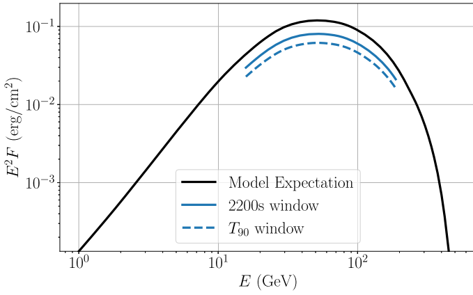
Figure 5. Sub-photospheric neutron-proton collision model and limits for GRB 221009A. (Left) All-flavor sub-photospheric model prediction for GRB 221009A assuming a Lorentz factor of \Gamma = 400 , an equivalent isotropic energy of 1.2 \times 10^{55} erg and neutron-proton opacity times baryon loading \xi_N \tau_{np} = 5 . GRECO-Astronomy 90% confidence level limits are during T_{90} and during a 2200 s time window that includes 200 s prior to the start of T_{90} (Abbasi et al. 2023b). (Right) Constraint on \xi_N \tau_{np} , as a function of the bulk jet Lorentz factor \Gamma for GRB 221009A. The model rejection factor (MRF) is the ratio of model signal event expectation to the 90% confidence level limit on the signal. We use the GRB 221009A limit from a time window of 2200 s. The region above the black solid line is rejected at a 90% confidence level. The canonical value of \xi_N \tau_{np} = 5 is shown as a dashed black line.
