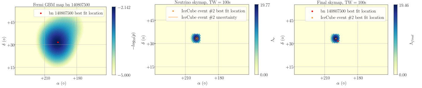
Figure 3. Three skymaps in equatorial coordinates. (Left) The HEALPix sky map of the Fermi-GBM GRB bn 140807500, the most significant GRB identified in this work. The best-fit location of bn 140807500 is that of P_{\max} on the GBM map. (Center) Neutrino sky map \Delta_{\nu} . The direction and location uncertainty of neutrino event #2 found in coincidence with bn 140807500 is shown. (Right) The neutrino and GRB final sky map \Delta_{\text{final}} , which is calculated from Equation (6).
