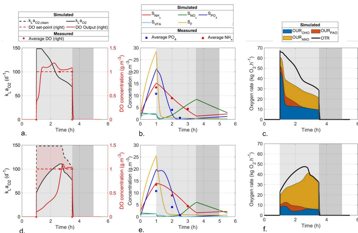
Figure 3. Simulation results of the model calibration at steady state with the average measured values of 14 batch cycles between 3-6 July, 2020 of the reference case for a constant maximum alpha=1 (top graphs, a-c) and a time-dependent alpha factor (bottom graphs, d-f). (a) and (d): simulated DO set-point ( \text{g.m}^{-3} ), PI controller's manipulated k_L a_{O_2, \text{clean}} , and the effective k_L a_{O_2} = \alpha F \cdot k_L a_{O_2, \text{clean}} ( \text{d}^{-1} ), controlled and measured DO concentration ( \text{g.m}^{-3} ). b and e: simulated and measured concentration profiles ( \text{g.m}^{-3} ). c and f: oxygen uptake rate (OUR, \text{kg O}_2.\text{h}^{-1} ) for different species (OHO, PAO, and ANO) compared to the oxygen transfer rate (OTR, \text{kg O}_2.\text{h}^{-1} ). The light grey shaded area represents the aeration phase, whereas the dark grey shaded area denotes the post-denitrification phase.
