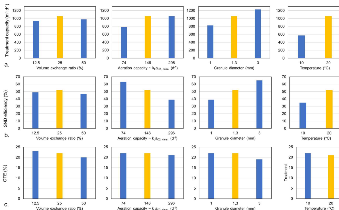
461 Figure 5. Overview of the different scenarios with dynamic alpha factor and their effect on (a) 462 the treatment capacity ( \text{m}^3 \cdot \text{d}^{-1} ), (b) simultaneous nitrification and denitrification (SND) 463 efficiency (%) and (c) the oxygen transfer efficiency (OTE, %). The reference case is marked 464 in yellow.
