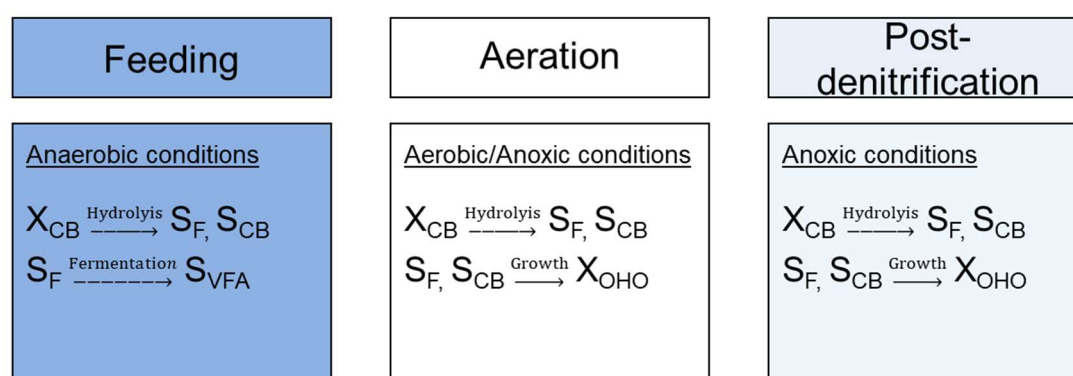
Figure 2. Visualization of the different biodegradable COD components, either particulates (X) or solutes (S), over the different batch phases, of the extended ASM2d model.
