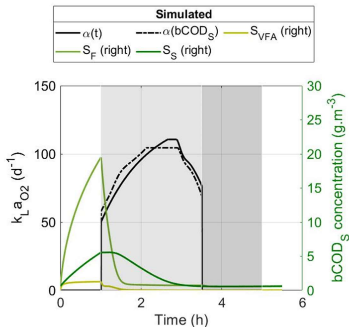
Figure 4. Simulated oxygen mass transfer coefficient ( k_{LaO_2} = \alpha F \cdot k_{LaO_2, \text{clean}} , d^{-1} ) for the alpha factor described by the time-dependent first-order relation ( \alpha F(t) ) compared to the alpha factor related to the soluble biodegradable organic carbon ( \alpha F(bCOD_S) ) determined by [15]. bCOD_S is defined as the sum of readily S_{VFA}(t) , S_F(t) and slowly biodegradable COD S_{CB}(t) of which the concentration profiles are shown on the right y-axes.
