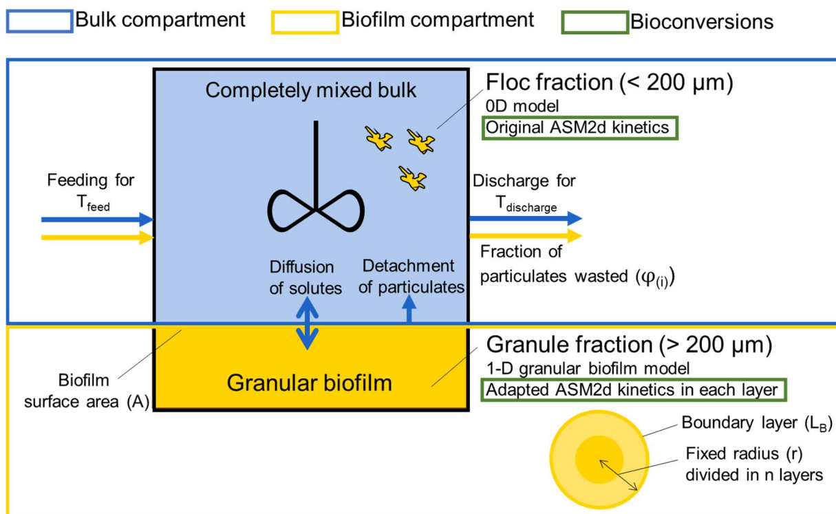
Figure 1. Schematic representation of the 1-D biofilm reactor model features developed in this study.
