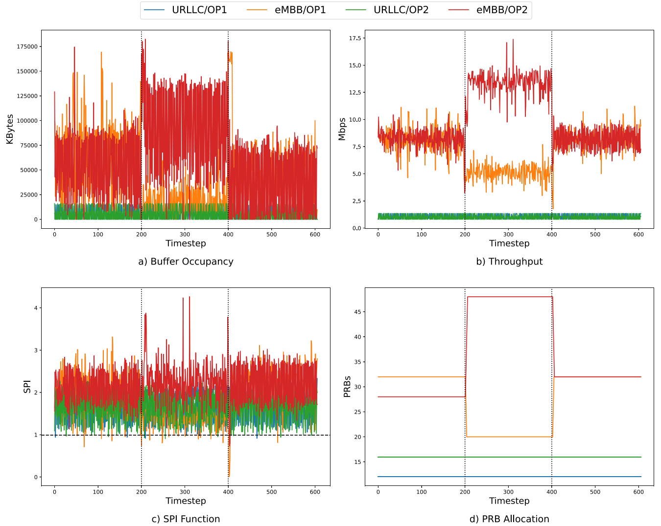
FIGURE 3. Metrics for each slice during the traffic scenario obtained using the deep Q-learning xApp. The x-axis represents timesteps after starting the traffic scenario, where each timestep corresponds to 250ms. The vertical dotted lines at t = 200 and t = 400 indicate the changes in the traffic scenario and metrics, while the horizontal dotted line in (c) represents the SLA violation threshold.
