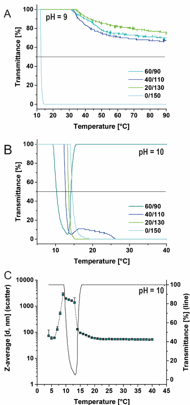
Figure 1. Response of C3DIPEDox-containing (co)polymers to pH value and temperature. Polymer concentration: 5 mg mL -1 in diH 2 O. Z-average was determined via DLS measurements. Transmittance was determined via turbidimetry measurements (Crystal16™). A and B: Turbidimetry curves of PC3DIPEDox 150 , PMeOx 20 - b -PC3DIPEDox 130 , PMeOx 40 - b -PC3DIPEDox 110 , and PMeOx 60 - b -PC3DIPEDox 90 at pH9 (A) and at pH 10 (B). C: Overlay of temperature-dependent Z-average and transmittance of PMeOx 60 - b -C3DIPEDox 60 at pH = 10.
