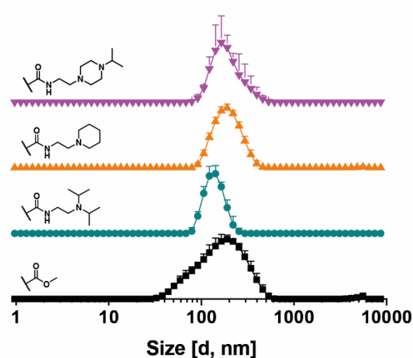
Figure 3. Size-distribution of polymer NPs. NPs were prepared from polymers and cargos at indicated concentrations via thin-film assembly in DMEM/F12 at 37 °C. NPs were analysed via DLS measurements at 37 °C (3 measurements with 3 runs each). Polymer concentration: 1 mg mL -1 . A: 5wt% RhB-C18; B: 5wt% RhB-C18 + 5 wt% Ptx.
