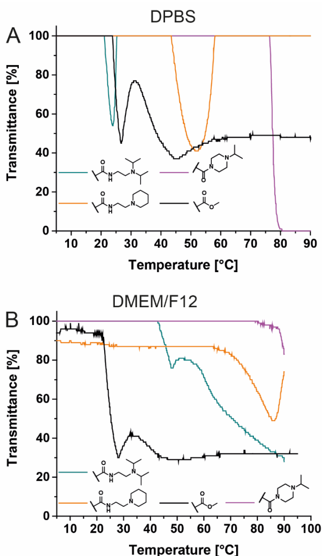
Figure 2. Temperature-dependent turbidity of different amine- and methyl ester-modified (co)polymers in DPBS (A) and DMEM/F12 (B). Polymer concentration: 5 mg \text{mL}^{-1} . Transmittance was measured via UV vis measurements (Crystal16™).
