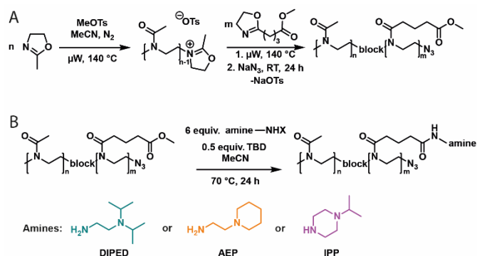
Scheme 1. Preparation of polymers used in this study. A: Synthesis of PMeOx n -b-PC3MestOx m via cationic ring-opening polymerisation of MeOx (1 st block) and sequential addition of C3MestOx (2 nd block), followed by termination with sodium azide. B: Post-polymerisation modification of PMeOx n -b-PC3MestOx m , yielding different tertiary amine-modified polymers.
