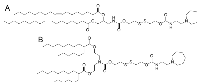
Figure 2. Molecular structure of the ionizable lipids (A) S-Ac7-Dog and (B) S-Ac7-DHDa.
