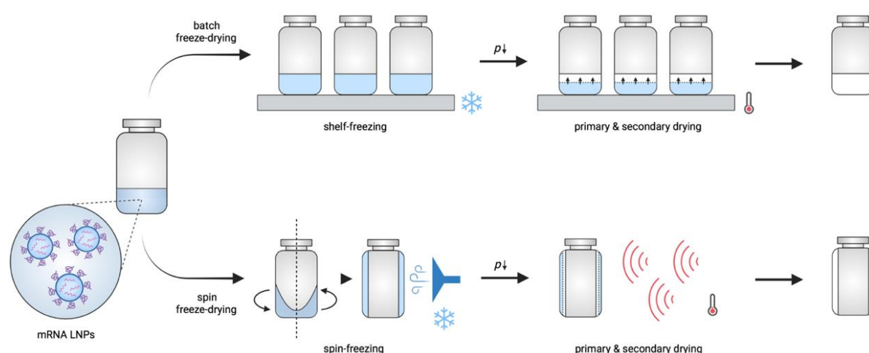
Figure 1. Schematic illustration of conventional batch freeze-drying and continuous spin freeze-drying
