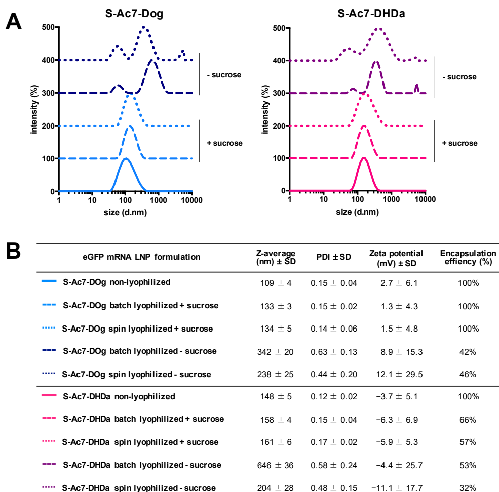
Figure 4. (A) Intensity-based size distribution curves measured by Dynamic Light Scattering (DLS) of S-Ac7-Dog (left) and S-Ac7-DHDa (right) eGFP mRNA LNP formulations. Curves are offset for clarity (B) Summarizing table of the biophysical properties of all mRNA LNP formulations.
