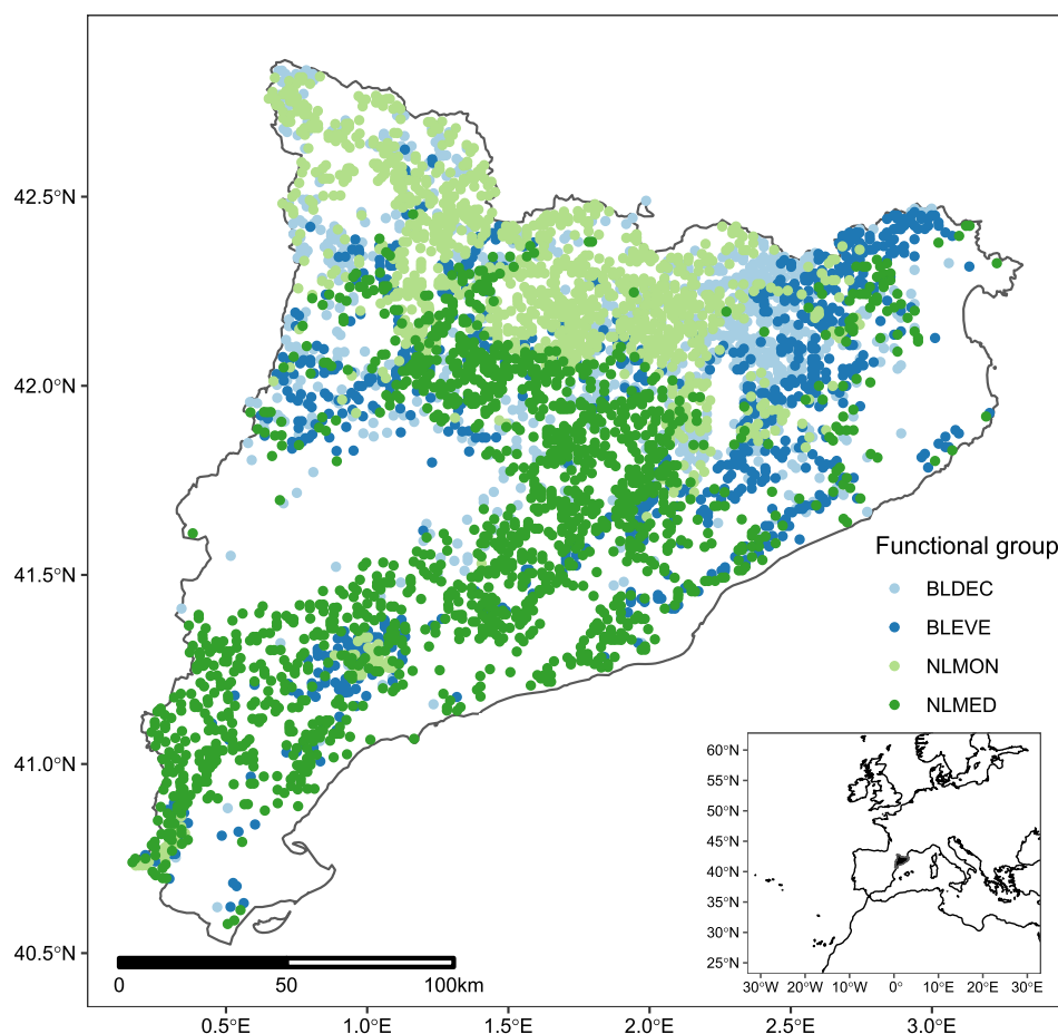
Figure 1. Study area. Map of Catalonia and the forest plots included in the analysis, with colored dots illustrating the functional group of the dominant species of each plot (light blue: BLDEC, broadleaf deciduous, dark blue: BLEVE, broadleaf evergreen, light green: NLMON, needleleaf montane, dark green: NLMED, needleleaf Mediterranean). Inset: the black area represents the location of the study area (Catalonia) within the Western Mediterranean Basin.
