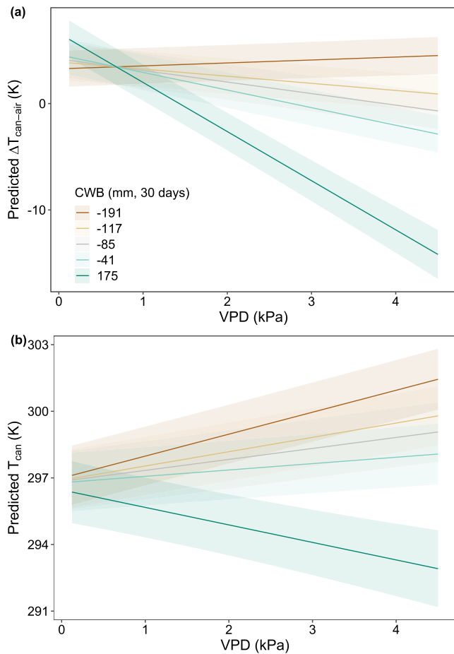
Figure 5. Interactive effects of vapor pressure deficit (VPD) and climatic water balance (CWB) on the thermal balance ( \Delta T_{can-air} ) and the canopy temperature ( T_{can} ). Model predictions of \Delta T_{can-air} (a) and T_{can} (b) as a function of the VPD and the climatic water balance (CWB) of the previous 30 days. Line colors illustrate different levels of CWB, from drier (negative) to wetter (positive) conditions. The shades around the lines correspond to the 95th confidence intervals of the predicted \Delta T_{can-air} . The interaction between VPD and CWB was significant in the mixed models.
