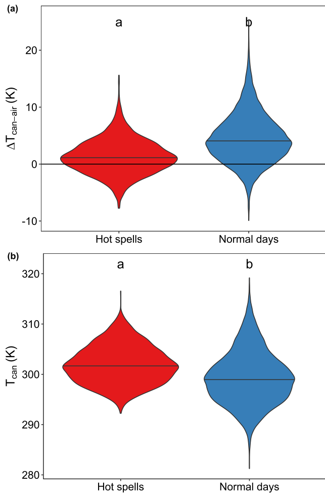
Figure 2. The thermal balance ( \Delta T_{can-air} ) (a) and canopy temperature ( T_{can} ) (b) in hot spells and normal days. For both \Delta T_{can-air} and T_{can} differences between hot spells and normal days were significant, as noted by the different letters above each group of data points.
