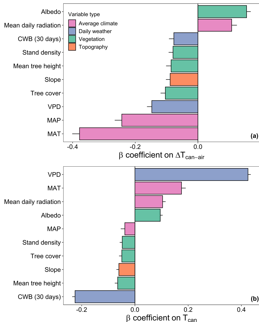
Figure 4. Drivers of the thermal balance ( \Delta T_{can-air} ) and the canopy temperature ( T_{can} ). Standardized \beta coefficients of the effect of the average climate (pink), daily weather (blue), forest structural (green) and topographical (orange) variables on \Delta T_{can-air} (a) and T_{can} (b). Positive (negative) coefficients on \Delta T_{can-air} imply correlations with warm (cool) T_{can} relative to T_{air} . Positive (negative) coefficients on T_{can} imply correlations with warmer (cooler) values of T_{can} . All variables included in the mixed model were significant ( p < 0.001 ). Uncertainty bars are the standard error of the mean, estimated for each individual effect. Effects are sorted based on their beta coefficient.
